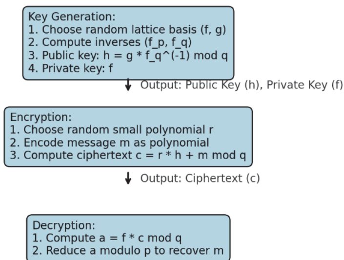
Fig. 2. Flowchart of Lattice –based RSA.
