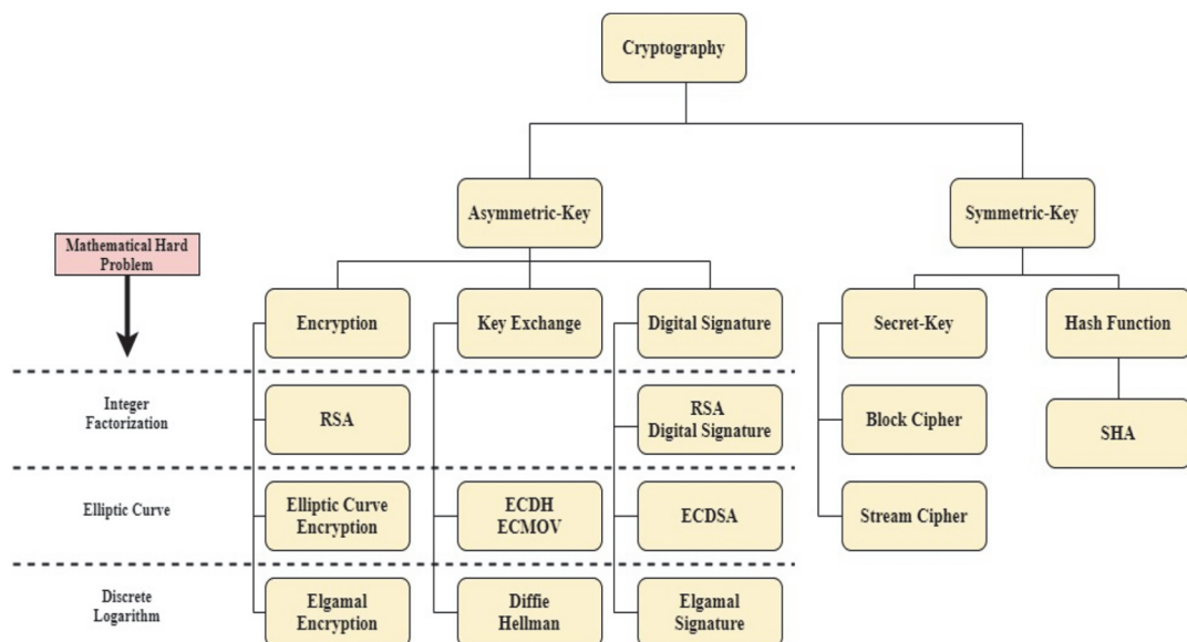
Fig. 1. Branches of cryptography and the related mathematical difficulties.
