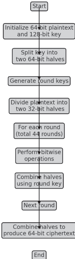
Fig. 3. Flowchart of SIMECK 64/128.
