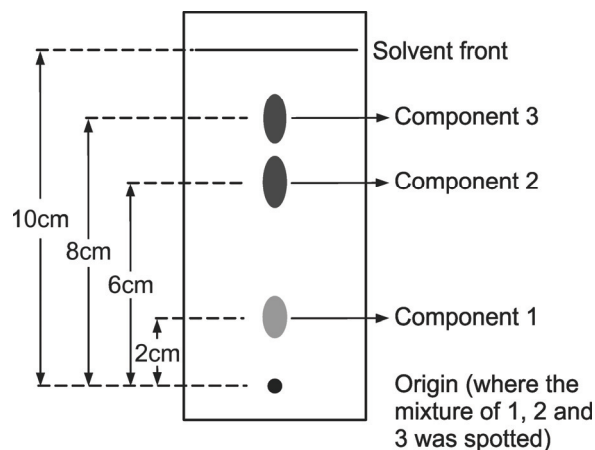
Fig. 1.2 Components of the mixture (referred by different numbers) travel at different rates
