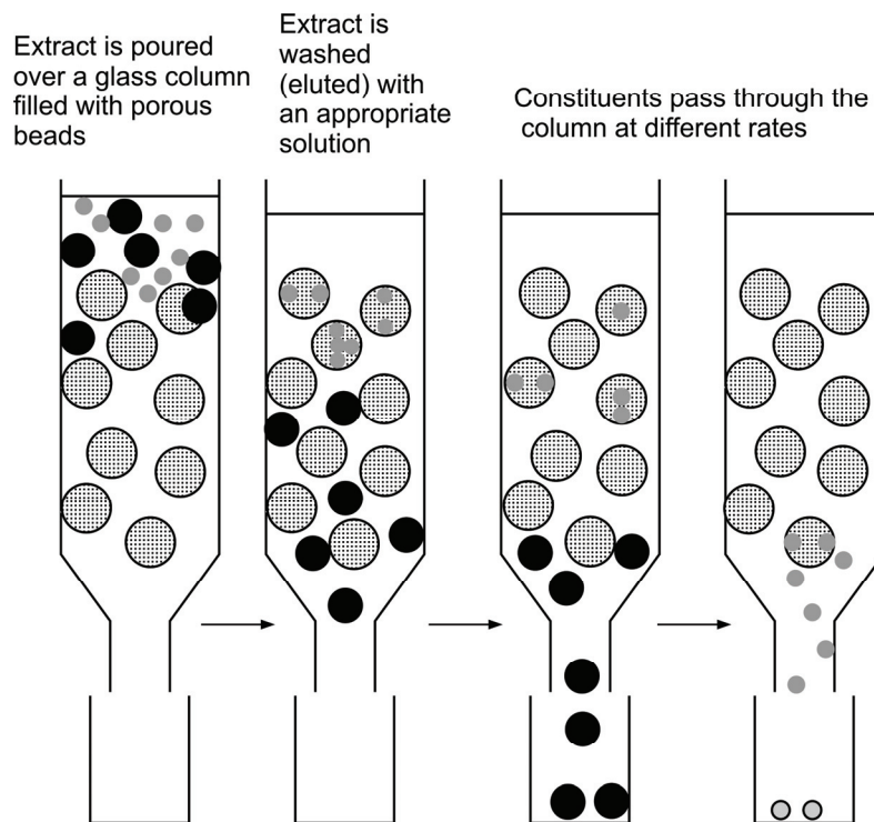
Fig. 1.5 Molecular Exclusion Chromatography. Differently sized macromolecules get separated at different times depending upon their molecular sizes
